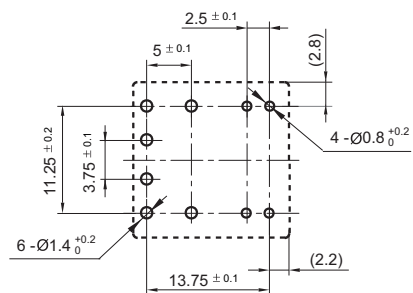
2 x Form C (Double relay)
