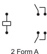
JQX-115F/ □□□□-□□-□-4-□□, 5mm Pinning, 2 Pole, 8A
