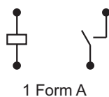
JQX-115F/ □□□□-□□-□-3-□□, 5mm Pinning, 1 Pole, 16A
